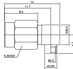
Right Angle Plug for UT085
