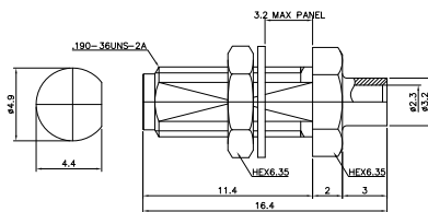
Bulkhead Jack for UT085
